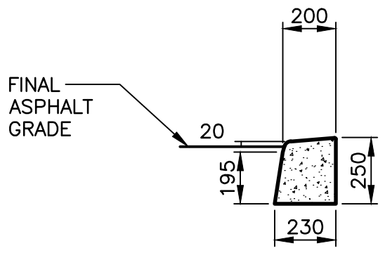
DEPRESSED CONCRETE CURB
