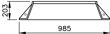
CONICAL GUIDE
