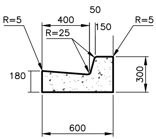
CONCRETE CURB & GUTTER
