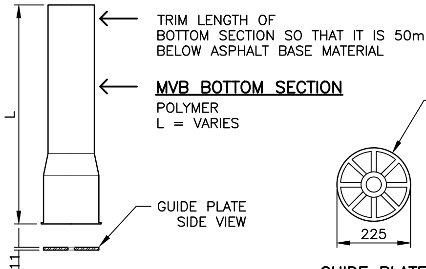
GUIDE PLATE DUCTILE IRON
