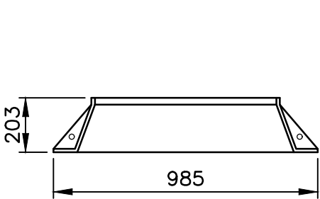
CONICAL GUIDE
