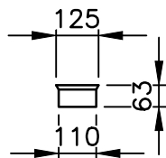
PLUG
