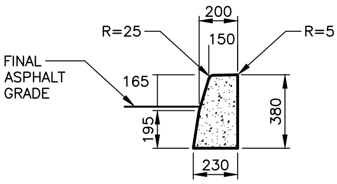
CONCRETE CURB
