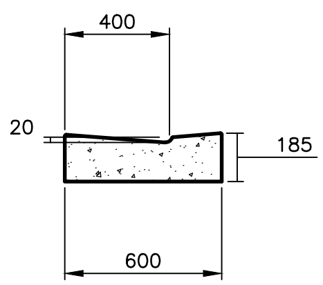
DEPRESSED CONCRETE CURB & GUTTER
